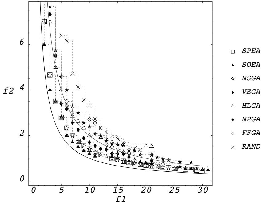
Figure 5: Test function T_5 (deceptive).
