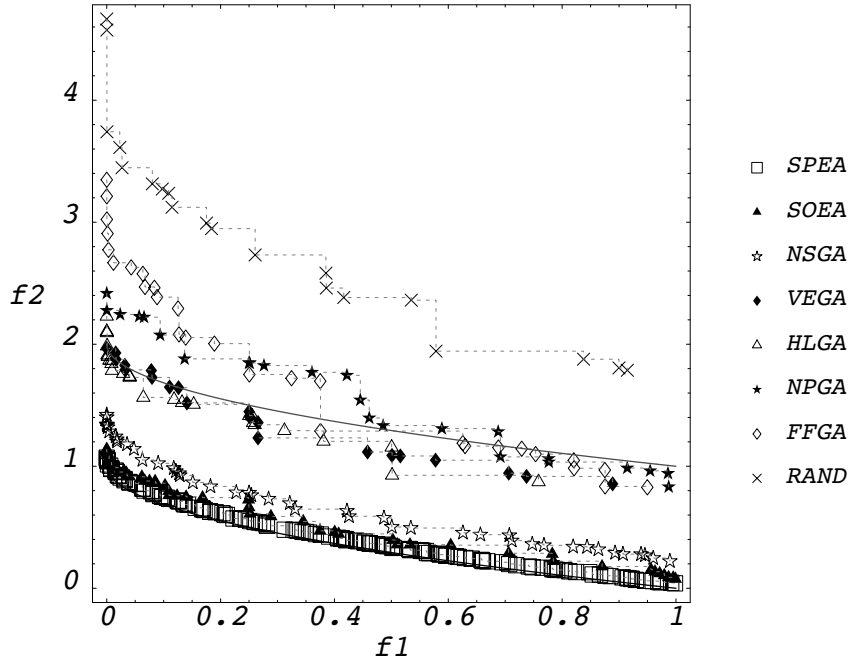
Figure 1: Test function T_1 (convex).
