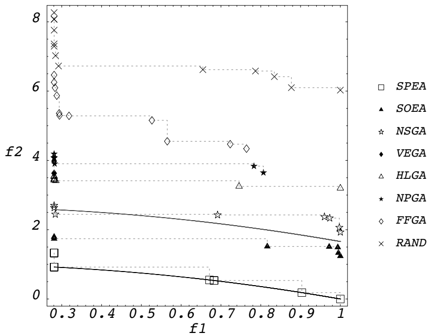
Figure 6: Test function T_6 (nonuniform).
