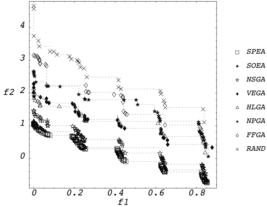
Figure 3: Test function \mathcal{T}_3 (discrete).
