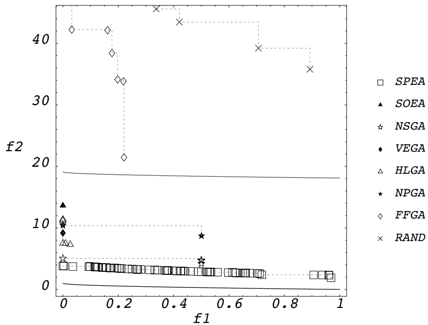
Figure 4: Test function \mathcal{T}_4 (multimodal).
