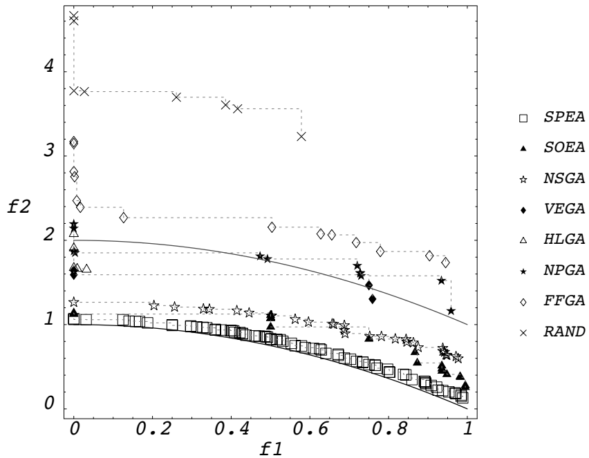
Figure 2: Test function T_2 (nonconvex).
